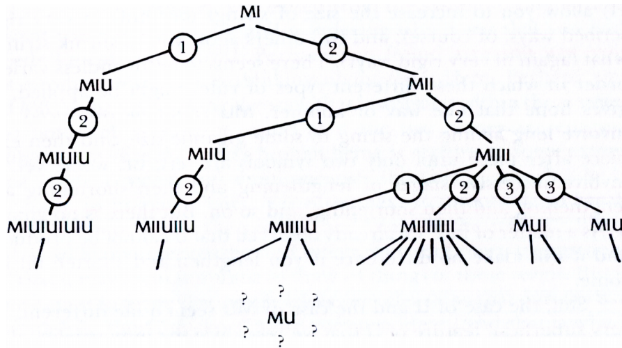
FIGURE 11. A systematically constructed "tree" of all the theorems of the MIU-system. The Nth level down contains those theorems whose derivations contain exactly N steps. The encircled numbers tell which rule was employed. Is MU anywhere in this tree?
