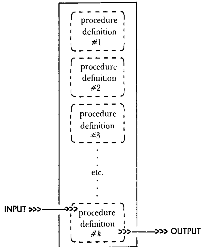
FIGURE 72. The structure of a call-less BlooP program. For this program to be self-contained, each procedure definition may only call procedures defined above it.
