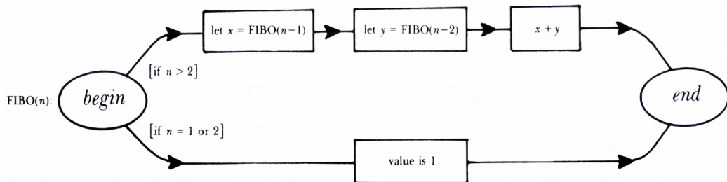
FIGURE 31. An RTN for Fibonacci numbers.
